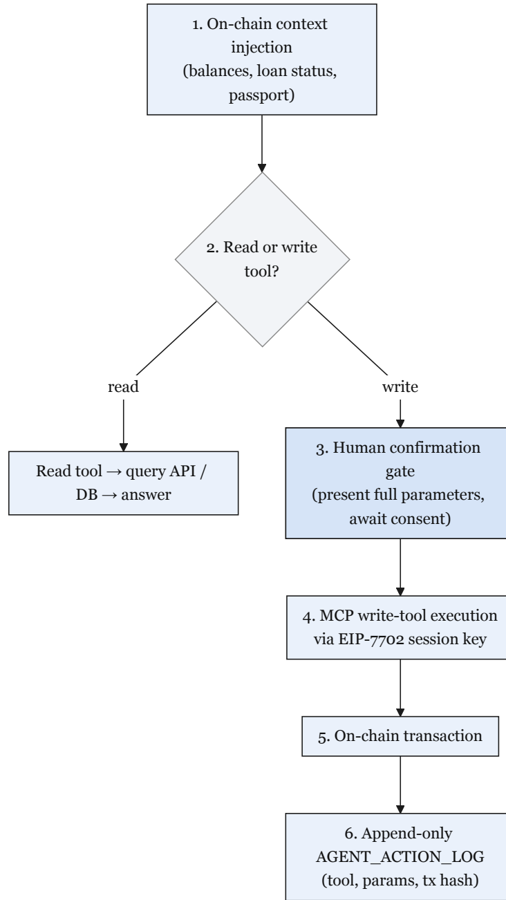
Figure 3.18: Conversational agent pipeline (Phase III MVT)
