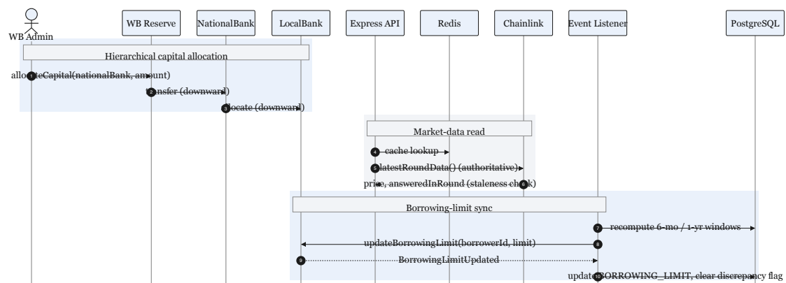
Figure 3.31: Sequence diagrams
