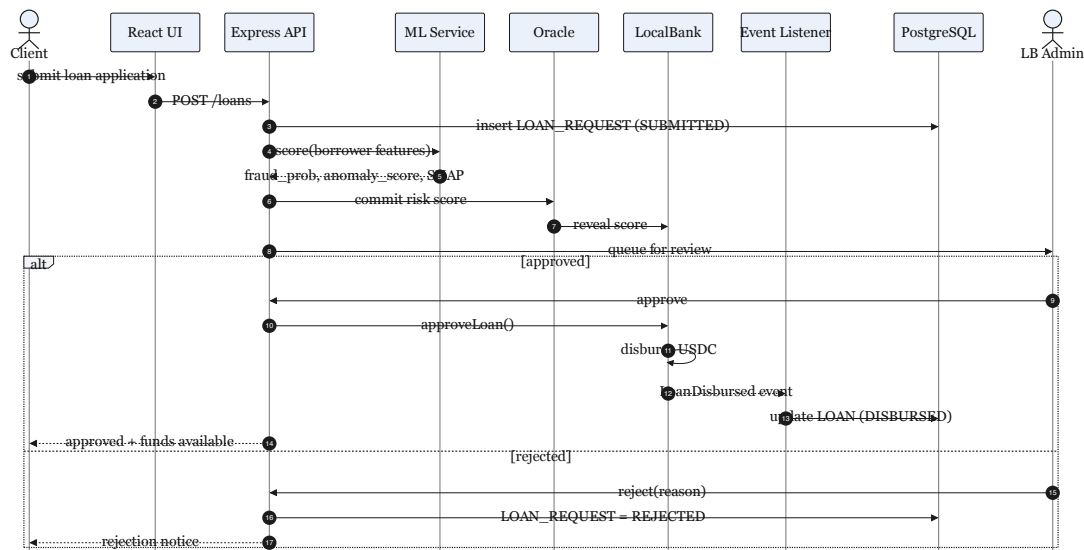
Figure 3.29: Loan approval sequence diagram
