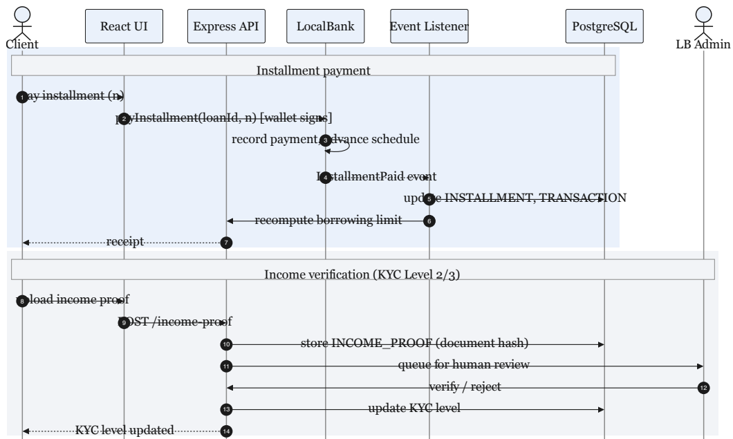
Figure 3.30: Sequence diagrams
